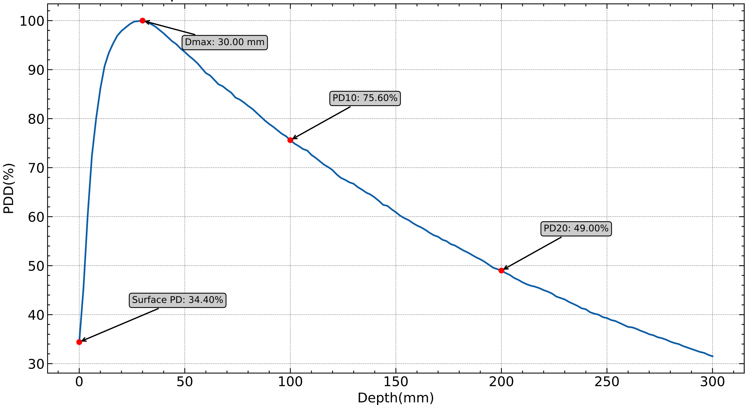
PDD profile of 15MV SSD=100, Water Phantom, F.S= 10x10cm 2
